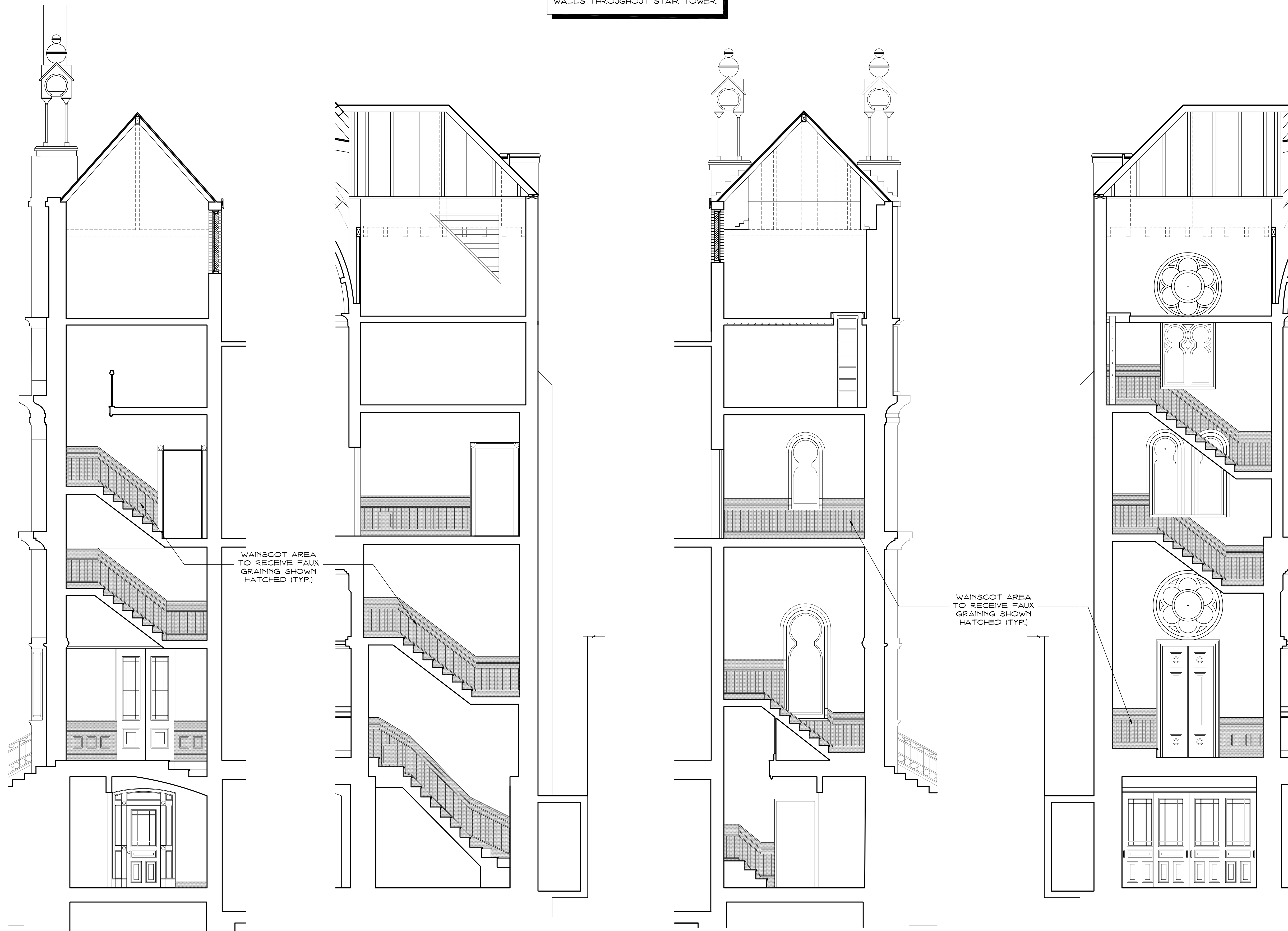
1 INTERIOR ELEVATION @ HISTORIC STAIR SCALE: 1/4" = 1'-0"
