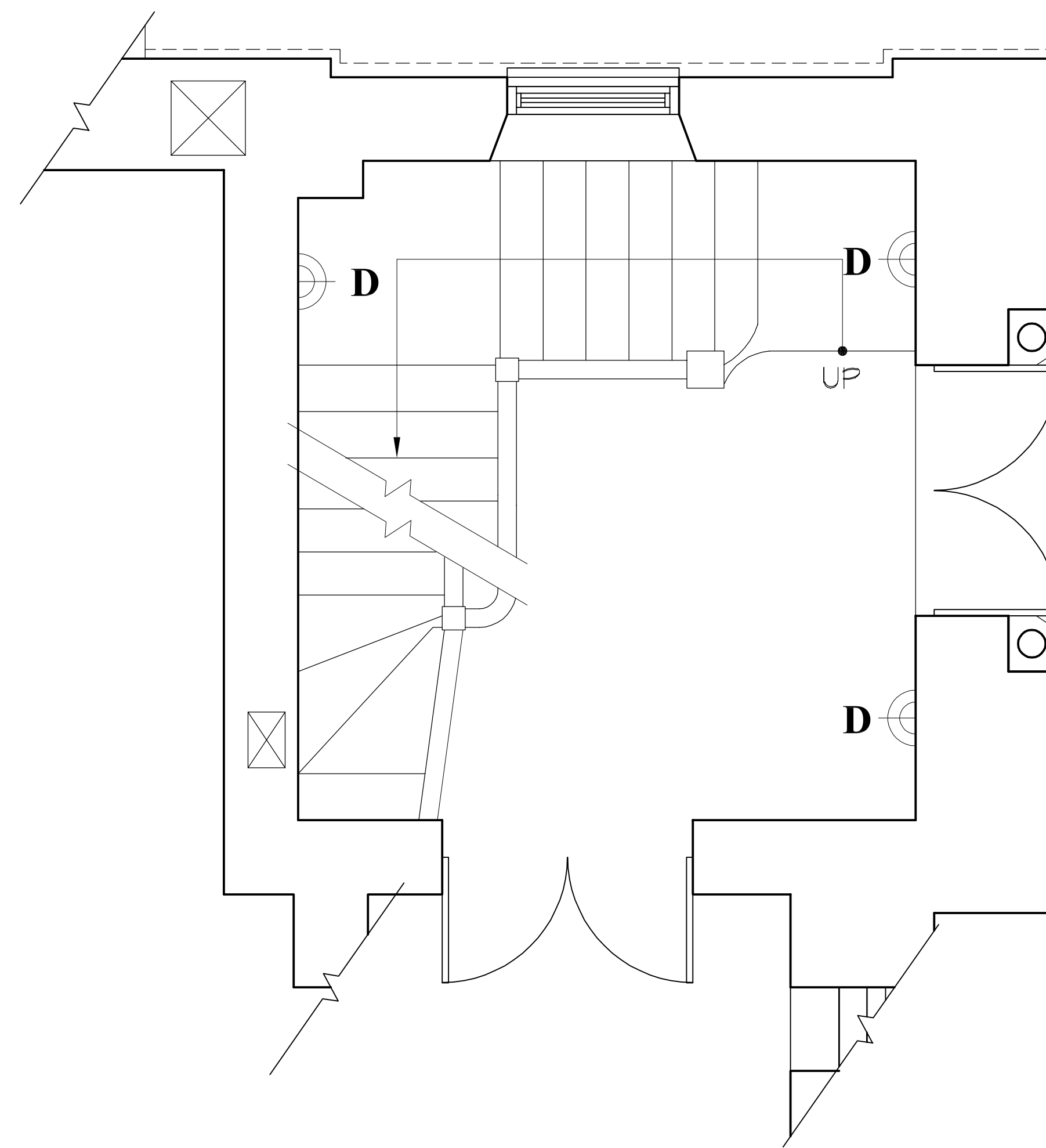
Stair Plan @ First Floor
