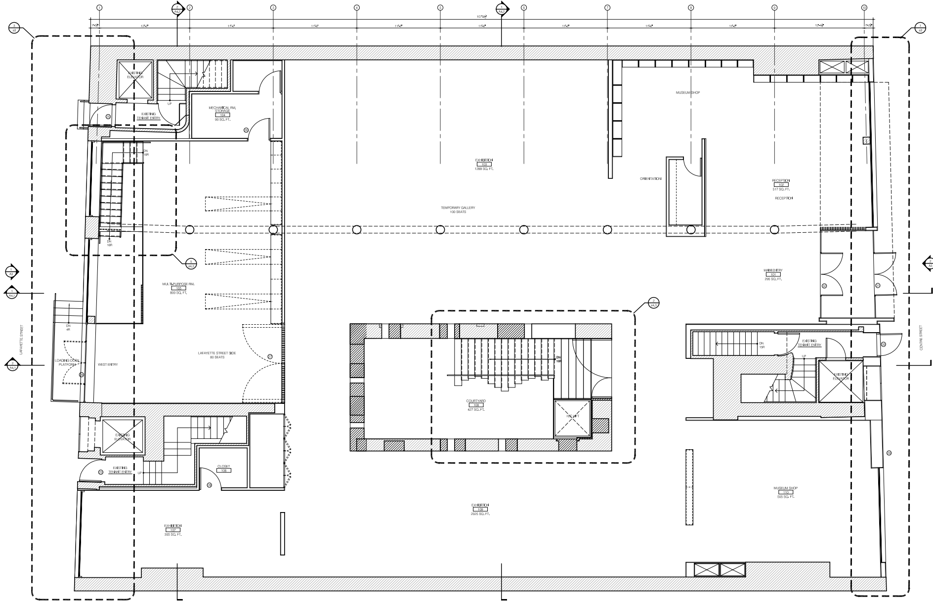
1 A2 PROPOSED GROUND FLOOR PLAN 1/2" = 1'-0"
